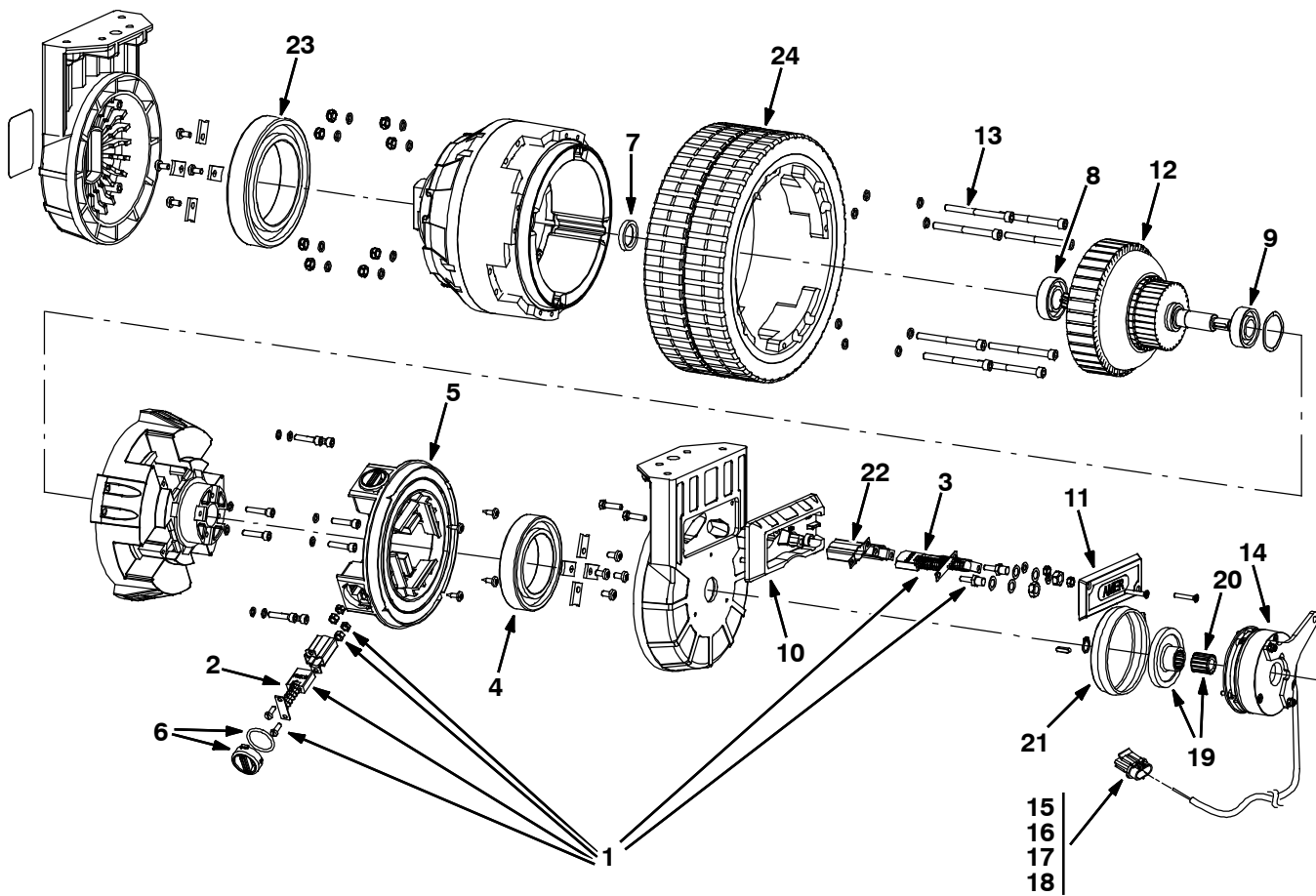
Fig. 12 - Front Wheel Gearbox Breakdown, 9001642, 9009000 (S/N 00000000-10518138)
