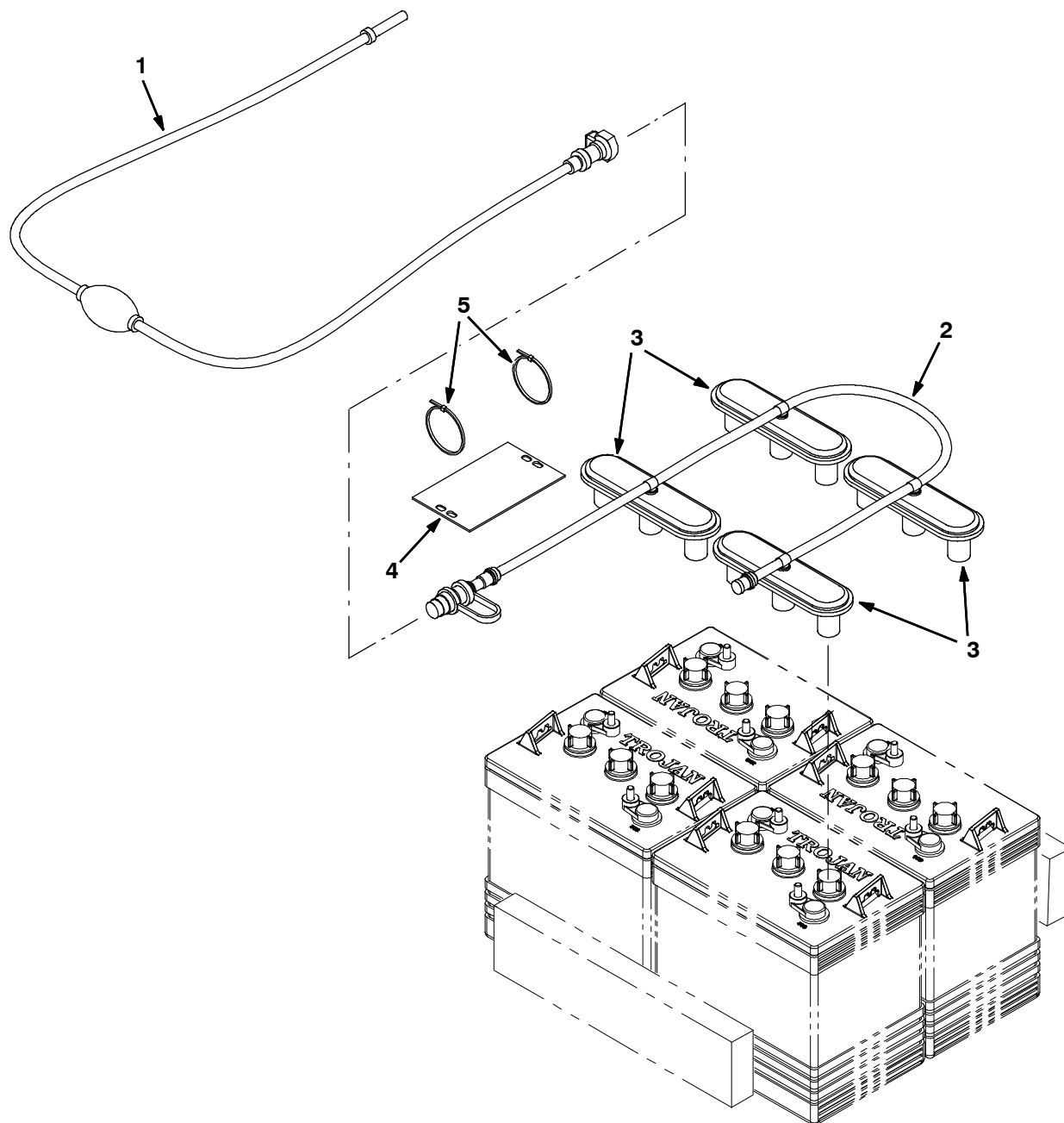
Fig. 18 - HydroLink® Battery Watering System Kit (S/N 10000000 - 11021175)
