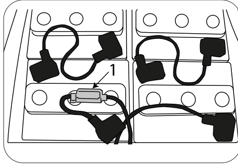
(Fig. 22-Ref.1) fusible general 100A.
