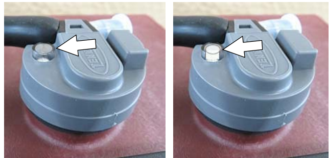
Low Float = Add Water High Float = Full FIG. 129
