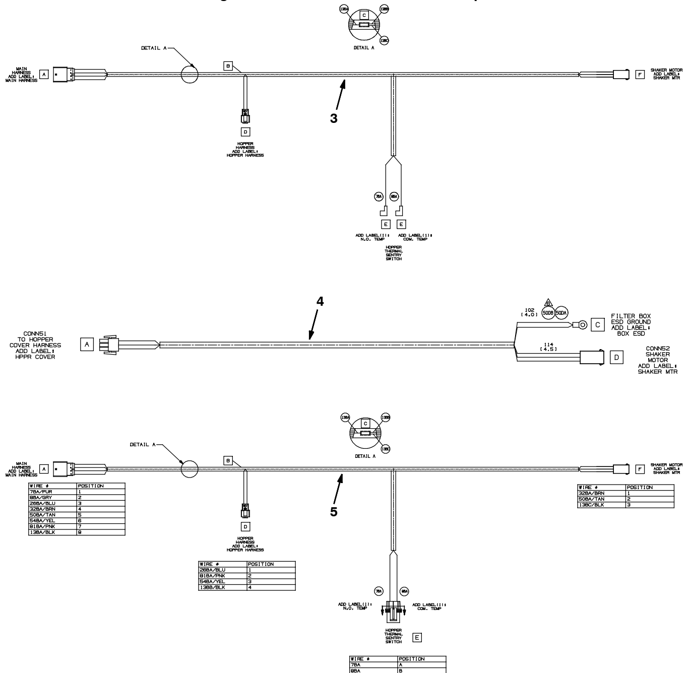
Fig. 45 - Electrical Wire Harnesses Group
