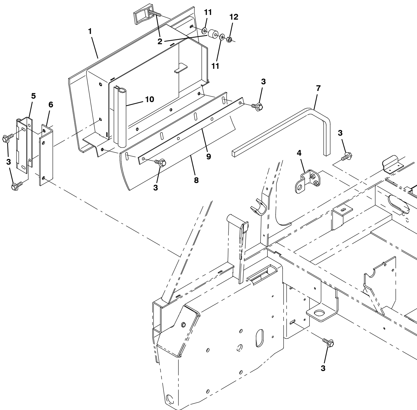
Fig. 3 - Brush Door Group, Right Side
