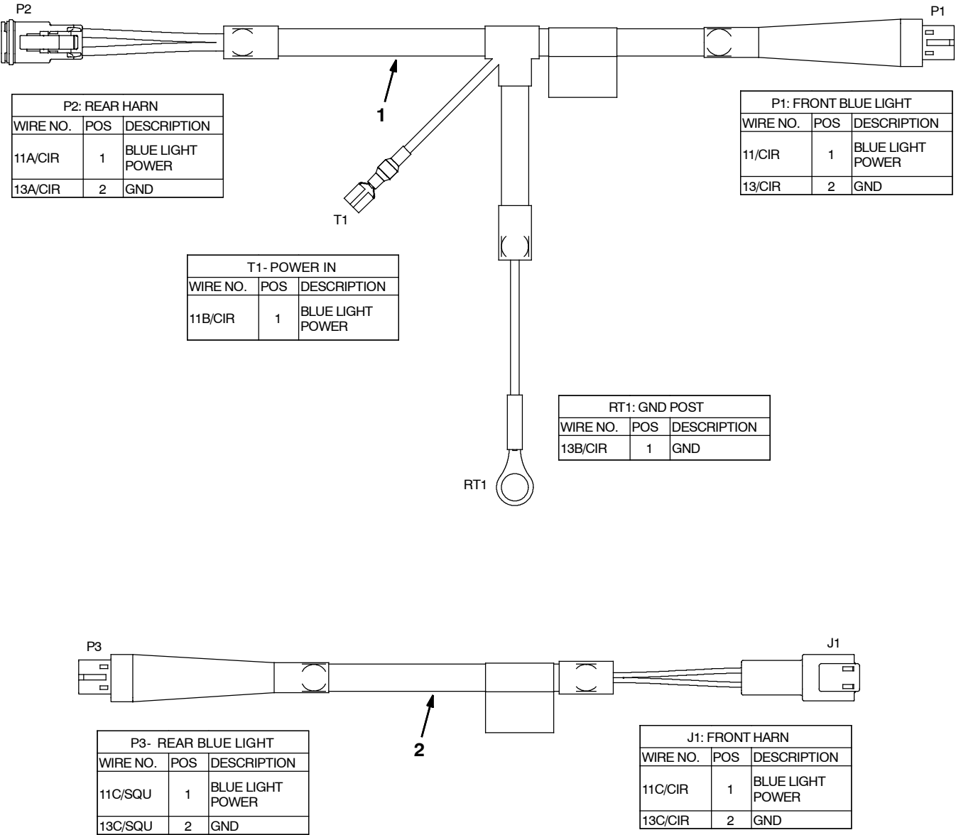
Fig. 40 - Spotlight Wire Harnesses Group
