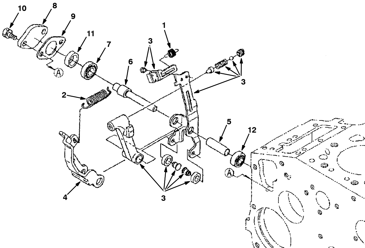
Fig. 18 - Governor Group
