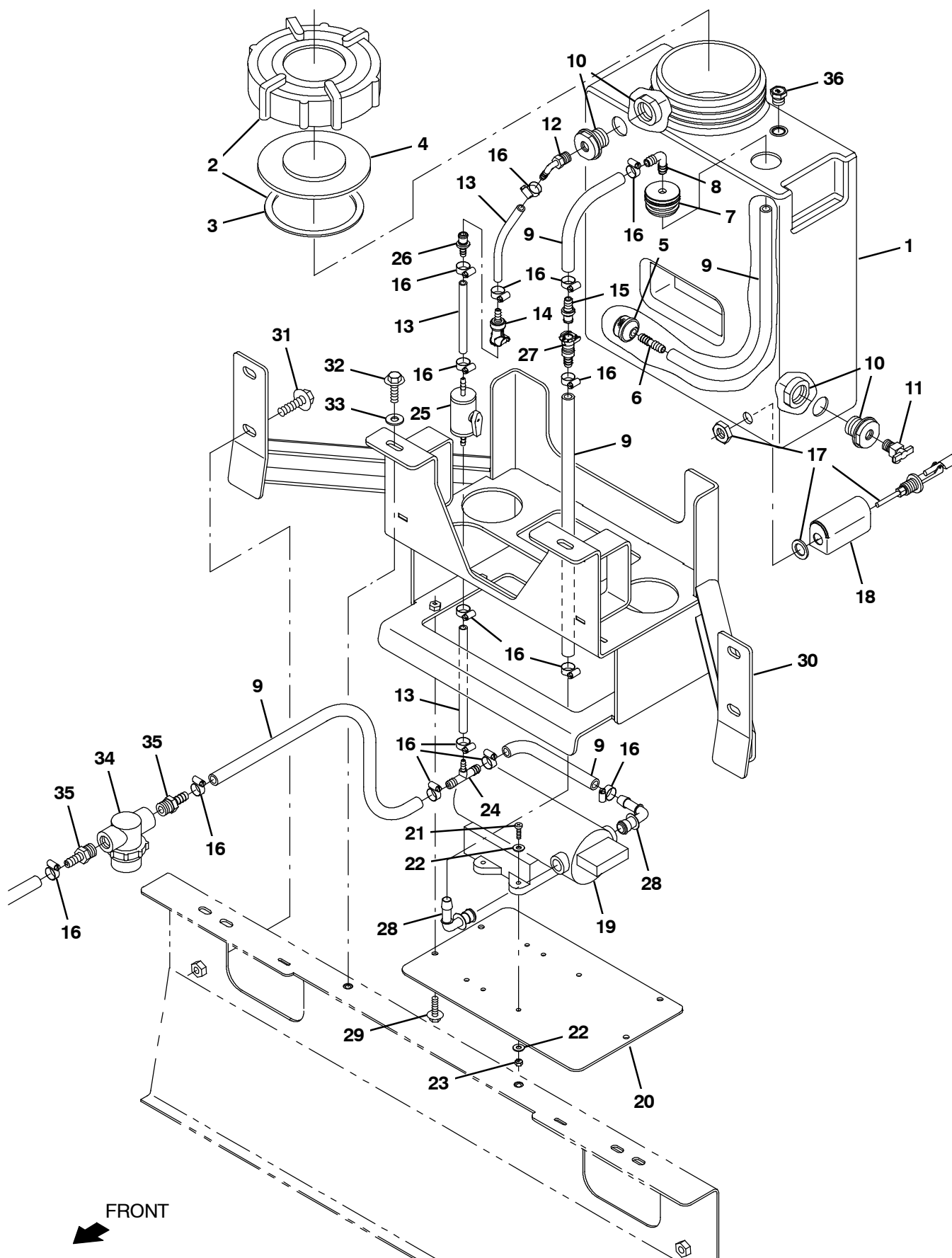
Fig. 31 - Wet Side Brush Dust Control Water Tank Group
