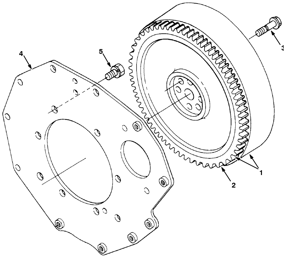
Fig. 14 - Flywheel Group
