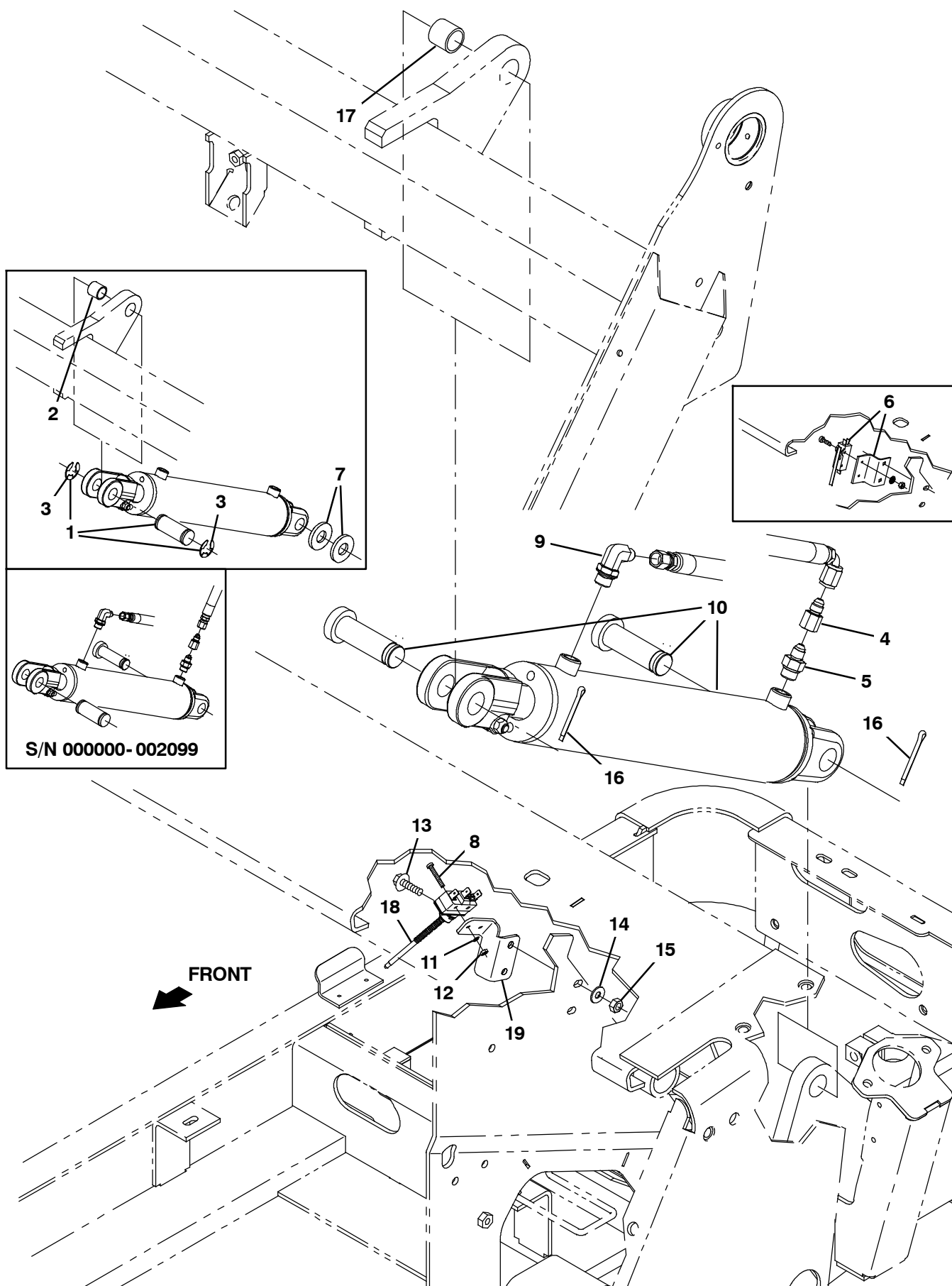
Fig. 28 - Hopper Lift Cylinder Group
